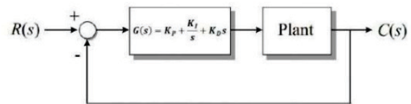
Fig.2. PID Control Block Diagram[5]
