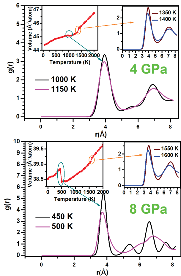
Fig. 4. Calculated g(r) 's for different temperature under 4 GPa and 8 GPa pressure.
