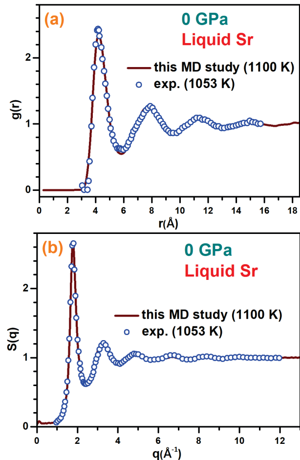
Fig. 2. Comparison of (a) g(r) and (b) S(q) calculated for liquid Sr with experimental results [12].
