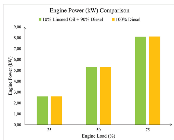
Fig. 2. Fuel and load-related changes in engine power
