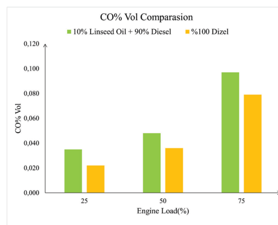
Fig. 4. Change in CO in engine exhaust emissions according to load and fuel type.
